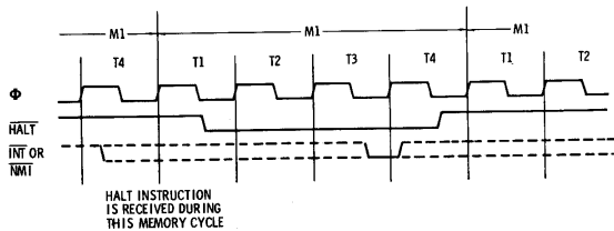
Fig. 3-11. Exit from HALT instruction.
