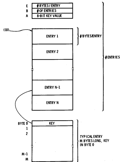
Fig. 16-3. Table search routine.
