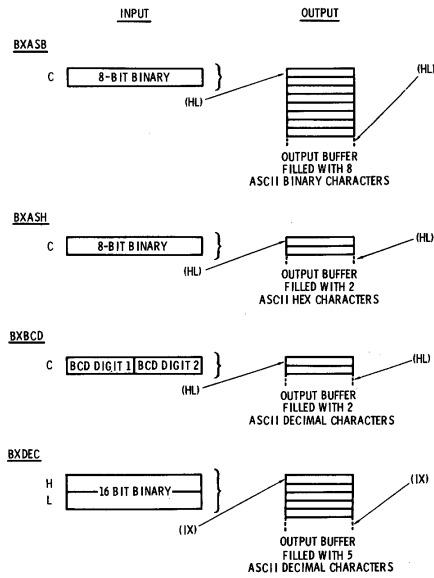
Fig. 16-2. Base X to ASCII conversions.
