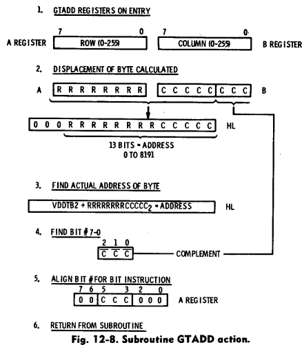
Fig. 12-8. Subroutine GTADD action.
