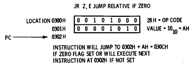
Fig. 4-16. Relative addressing in JR Z,E instruction.
