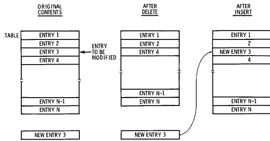
Fig. 13-5. Modify table entry actions.
