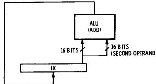
Fig. 5-14. Sixteen-bit arithmetic instruction examples.
