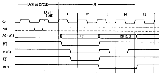
Fig. 3-10. Nonmaskable Interrupt Request cycle.
