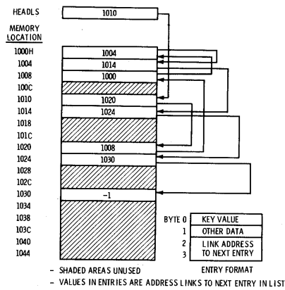
Fig. 13-8. Typical single-ended linked list.
