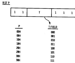
Fig. 5-22. RST P instruction.
