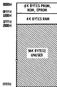
Fig. 17-3. Z-80 MCB™ nominal memory mapping.
