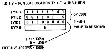
Fig. 4-18. Indexed addressing example.
