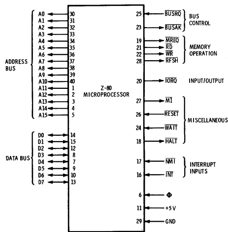
Fig. 3-1. Z-80 interface signals.
