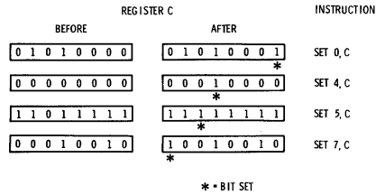
Fig. 4-20. Bit addressing example.
