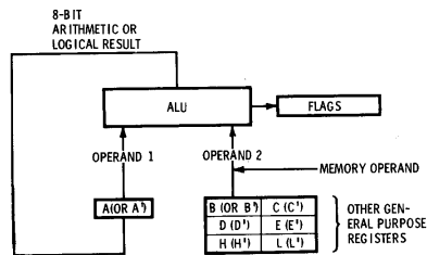
Fig. 2-3. Arithmetic and logical operations.
