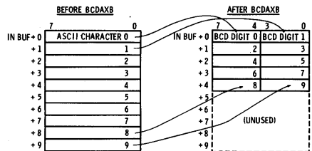
Fig. 12-5. ASCII to bcd conversion.
