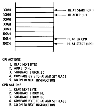
Fig. 5-8. CPI and CPD instructions.
