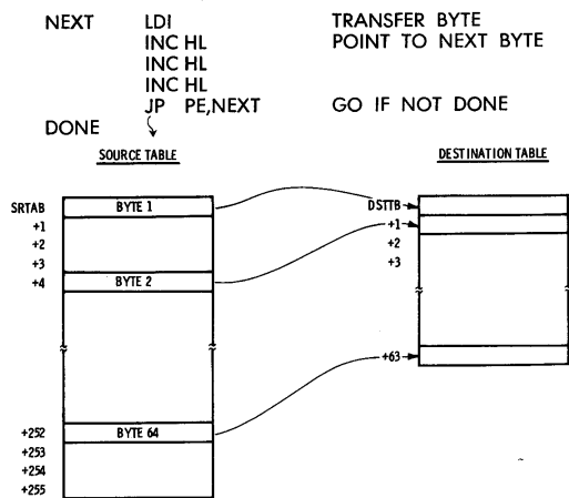
Fig. 10-4. Moving noncontiguous data with LDI.
