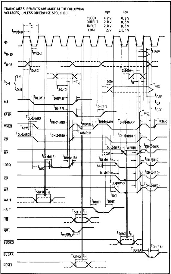
Fig. A-3. Z-80 ac timing diagram.
