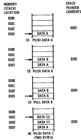
Fig. 2-8. Stack Pointer (SP) operation.
