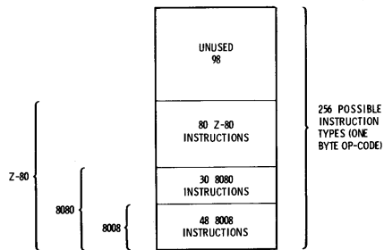
Fig. 1-2. Instruction comparison 8008, 8080, and Z-80.
