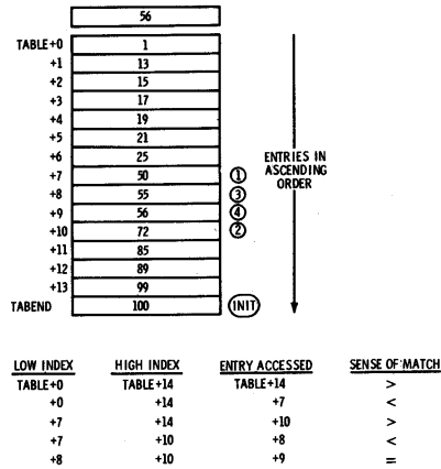
Fig. 13-7. Binary search example.
