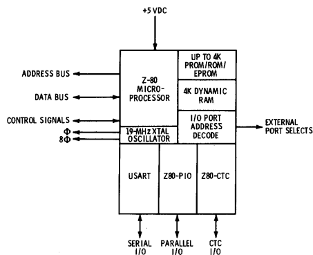
Fig. 17-2. Z-80 MCB™ functional block diagram.
