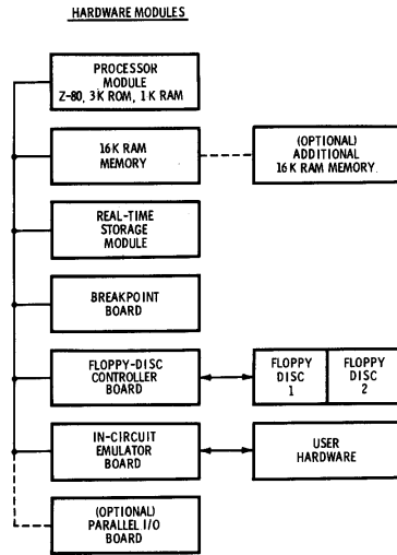
Fig. 17-5. Zilog Z-80™ development system.
