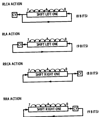
Fig. 5-15. RLCA, RLA, RRCA, RRA instructions.
