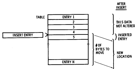
Fig. 13-4. Insert table entry actions.
