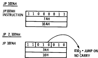
Fig. 5-20. JP and JPCC instruction examples.
