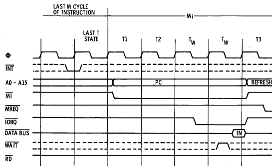
Fig. 3-9. Interrupt Request/Acknowledge cycle.
