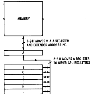
Fig. 10-3. A register used for random addressing.
