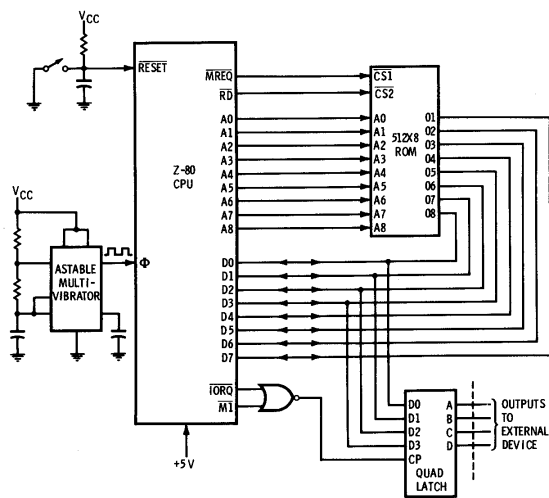
Fig. 8-1. A minimum Z-80 system.
