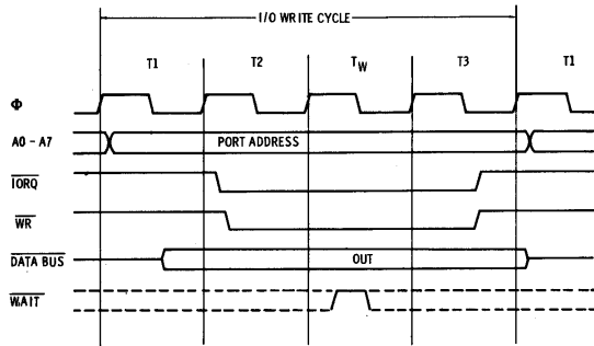
Fig. 3-7. I/O Write cycle.
