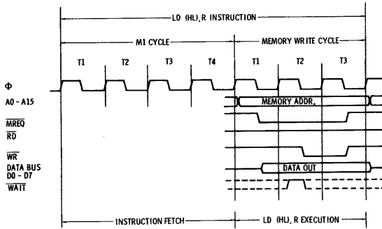
Fig. 3-5. Write cycle.
