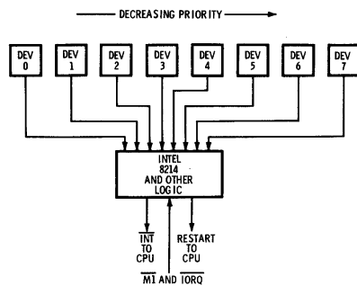
Fig. 7-4. Priority encoding for interrupt mode 0.
