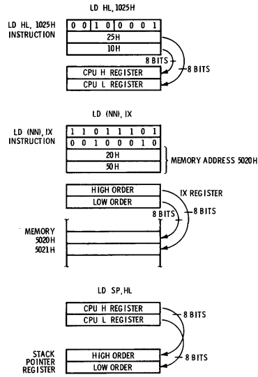
Fig. 5-2. Sixteen-bit load group examples.
