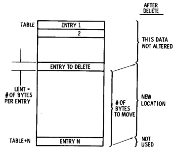
Fig. 13-3. Delete table entry actions.
