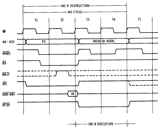
Fig. 3-3. M1 (op code fetch) cycle.
