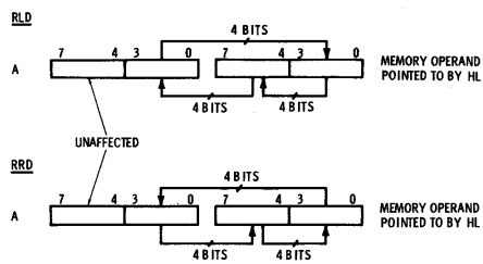
Fig. 12-4. RLD, RRD action.
