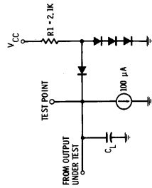
Fig. A-2. Load circuit for output.
