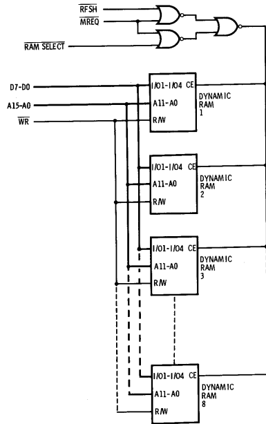
Fig. 8-5. Dynamic RAM refresh.
