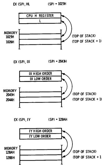
Fig. 5-5. EX (SP) instructions.
