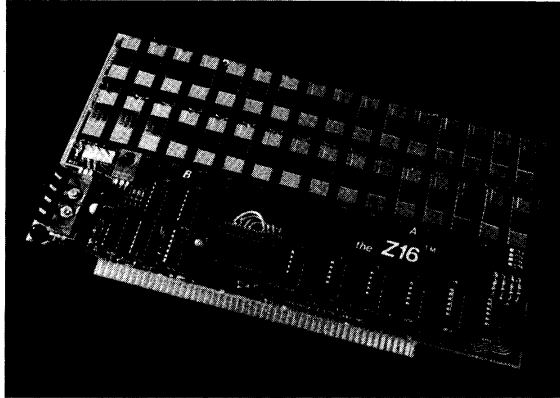
Fig. 18-2. TDL Z-16™ board.
