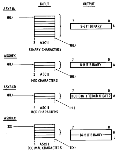
Fig. 16-1. ASCII to base X conversions.
