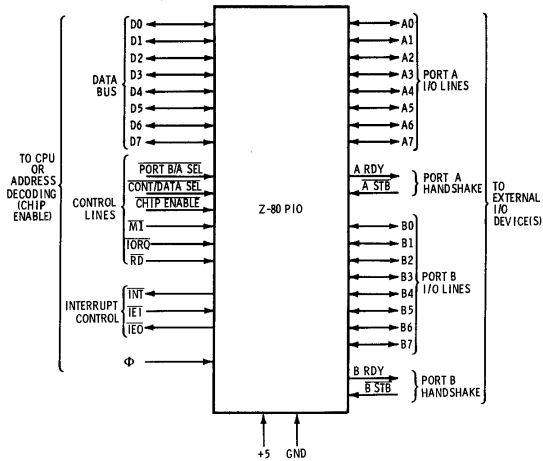
Fig. 8-6. PIO interface signals.
