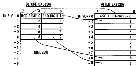
Fig. 12-6. Bcd to ASCII conversion.
