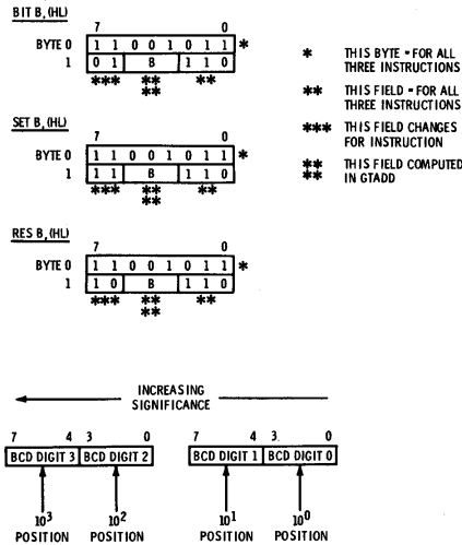
Fig. 11-2. Four-digit bcd representation.
