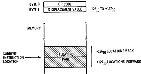
Fig. 4-15. Relative addressing.
