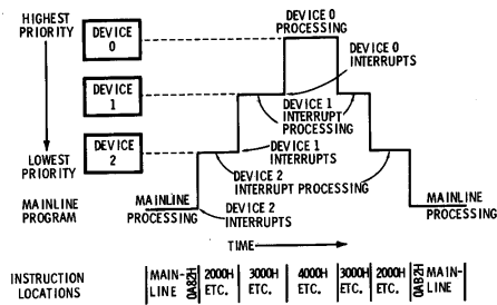
Fig. 7-8. Nested interrupt example.
