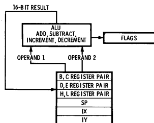
Fig. 2-5. Register pair double-precision operation.
