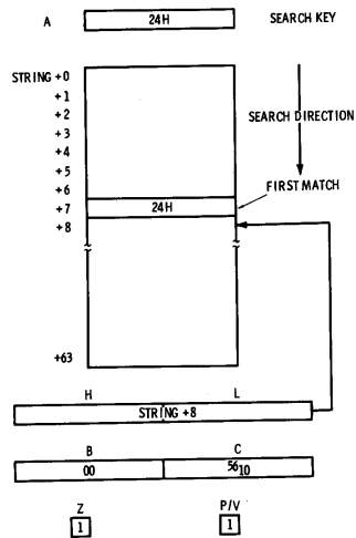
Fig. 13-1. String search terminating conditions.
