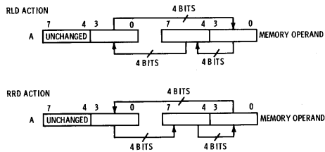
Fig. 5-16. RLD and RRD instructions.
