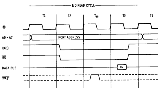
Fig. 3-6. I/O Read cycle.
