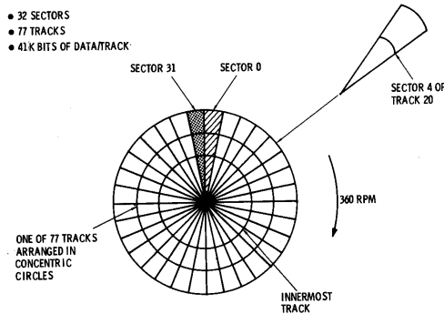
Fig. 15-1. Typical floppy-disc characteristics.
