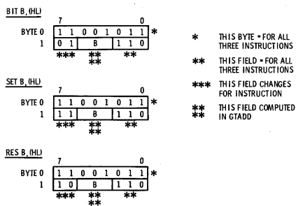
Fig. 12-9. Instruction modification for VDT bit routine.
