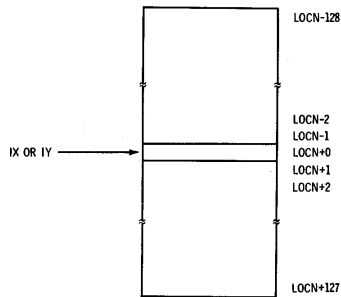
Fig. 10-1. Index register block access.
