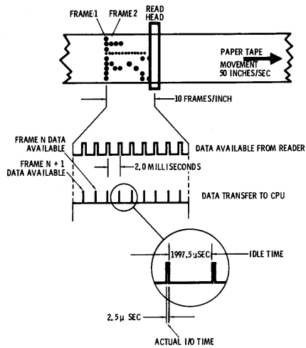
Fig. 7-1. I/O idle time example.
