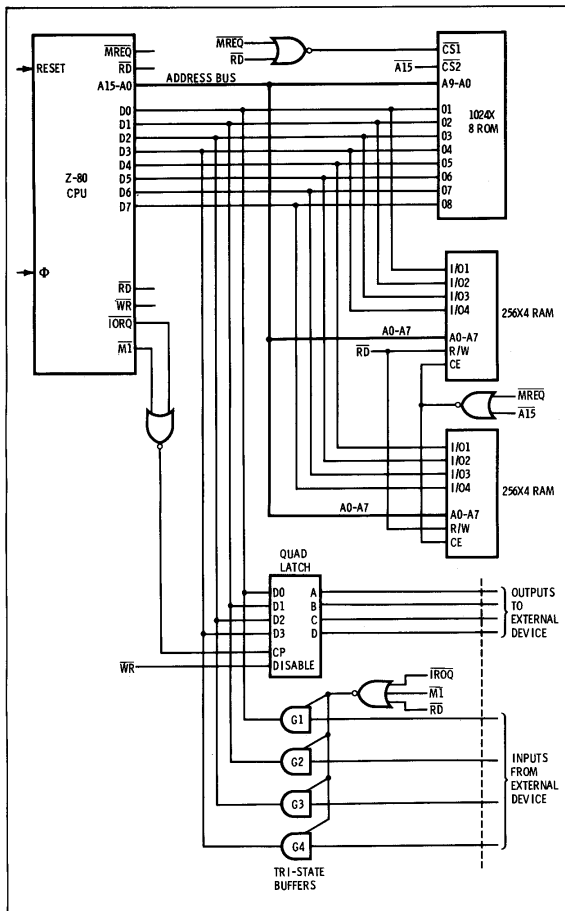
Fig. 8-2. Z-80 interfacing with RAM and ROM.
