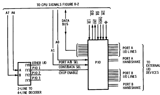
Fig. 8-12. PIO use in minimum configuration system.
