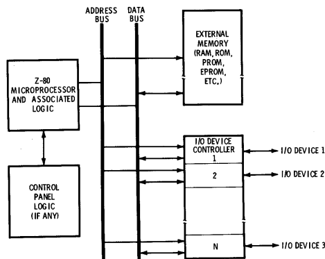
Fig. 2-10. Z-80 Microcomputer system component parts.
