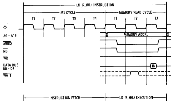
Fig. 3-4. Read cycle.
