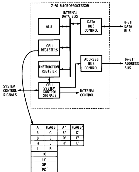
Fig. 2-1. Z-80 Microprocessor architecture.
