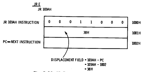
Fig. 5-21. JR E instruction example.
