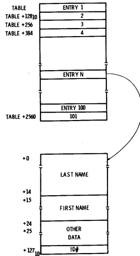
Fig. 13-2. Employee table format.
