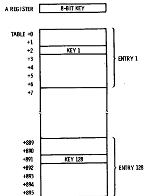
Fig. 11-1. Table search example.
