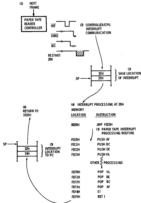
Fig. 7-3. Mode 0 interrupt processing.
