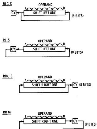
Fig. 5-18. RLC, RL, RRC, RR instructions.
