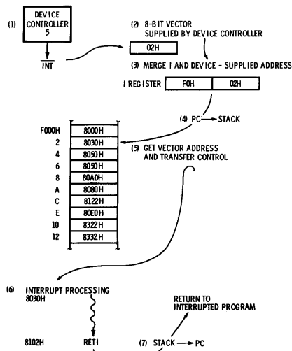
Fig. 7-6. Interrupt mode 2 example.
