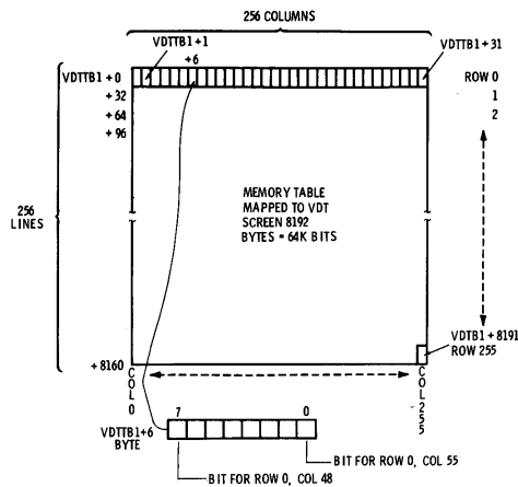
Fig. 12-7. VDT bit map for 64K pixels.
