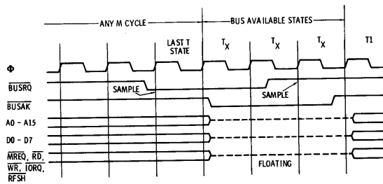
Fig. 3-8. Bus Request/Acknowledge cycle.
