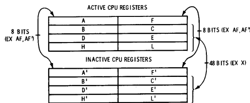
Fig. 5-4. EX AF,AF'; EX X instructions.
