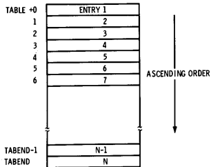
Fig. 13-6. Table for binary search example.
