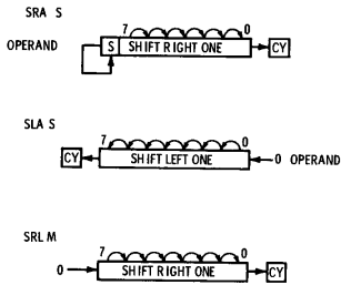
Fig. 5-17. SRA, SLA, SRL instructions.
