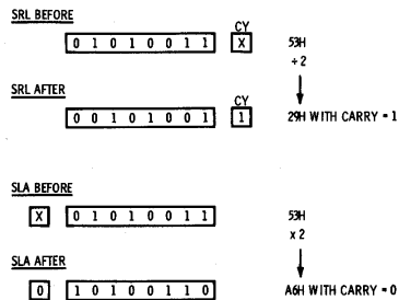
Fig. 12-1. Multiplication and division by shifting.
