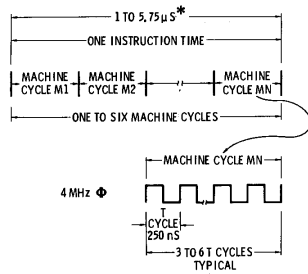
Fig. 3-2. Basic instruction cycles.
