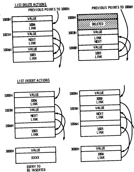
Fig. 13-9. List delete and insert actions.
