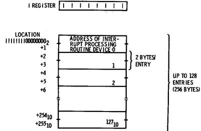
Fig. 7-5. Interrupt mode 2 interrupt vector table.
