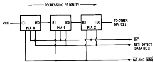
Fig. 7-7. Z-80 interrupt prioritizing interrupt mode 2.
